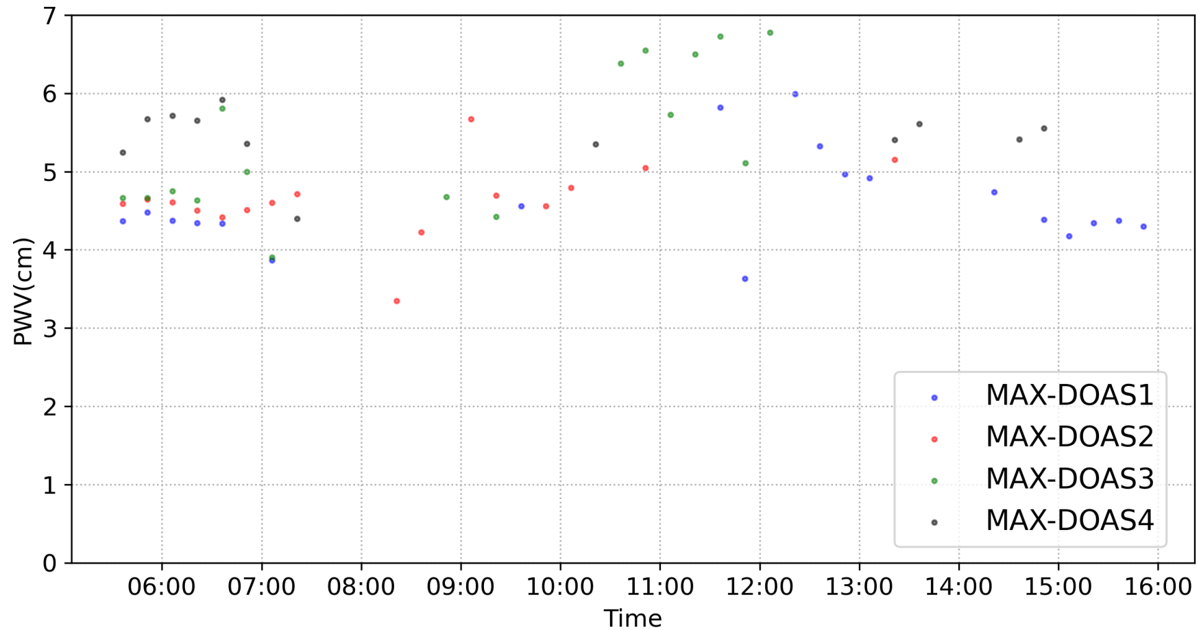
PWV(cm) of MAXDOAS1-4 in Chiba 2021/08/03
